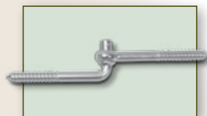
HSE6000C (5/8" x 5") Screw Hook & Eye Cadmium
